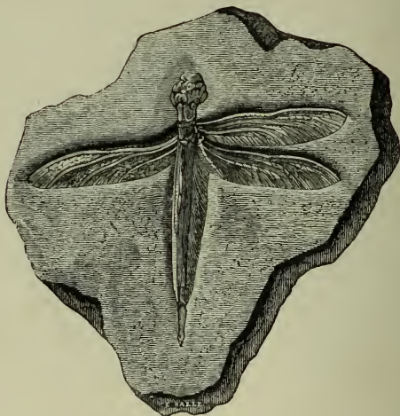
Fig. 7.—Fossil Dragon-fly of the Secondary Epoch.
